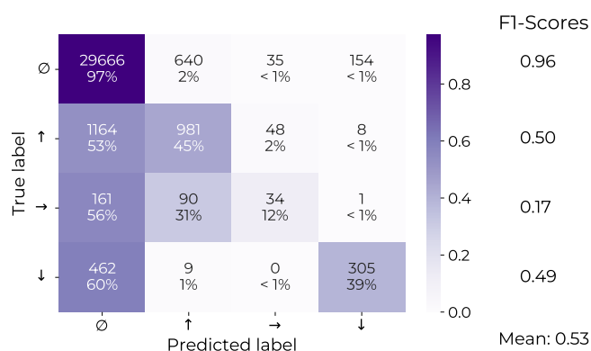
Figure 6.17: Confusion Matrix of the predictions of the MLP model on the same test set as the decision trees, with a threshold of 0.5.
